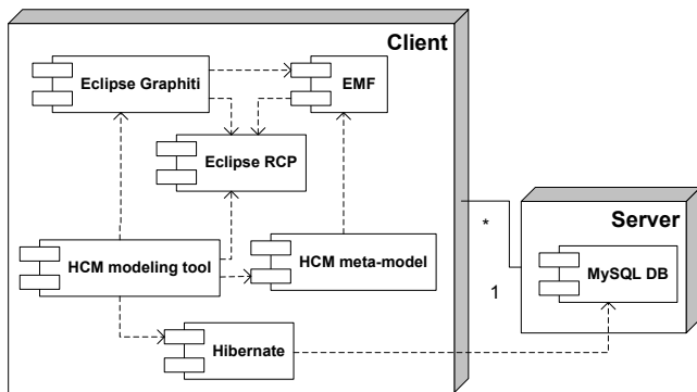
Figure 4. Client-server architecture of the HCM modeling prototype
